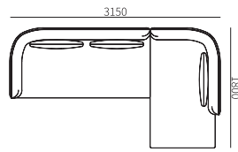
31F011ZH-02 3150*1800*680mm 124.0*70.9*26.8"
