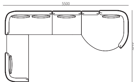
31F011ZH-08 5500*3150*880mm 216.5*124.0*34.6"
