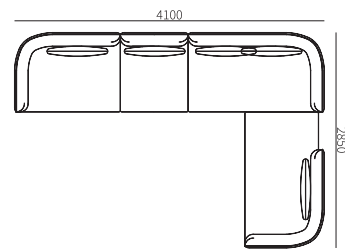
31F011ZH-06 4100*2850*680mm 161.4*112.2*26.8"
