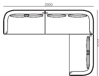
31F011ZH-05 3900*2850*680mm 153.5*112.2*26.8"
