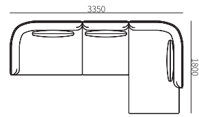
31F011ZH-03 3350*1800*680mm 131.9*70.9*26.8"
