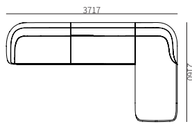
D02ZH-5 3717*2160*810mm 146.3*85.0*31.9"
