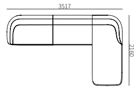
D02ZH-3 3517*2160*810mm 138.5*85.0*31.9"
