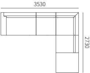
L186A-2R + L186B-1 + L186D + L186E-2L 3530*2730*720MM 139.0*107.5*28.3"
