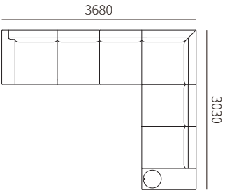
L186A-3R + L186E-2L + L186B-4 3680*3030*720MM 144.9*119.3*28.3"
