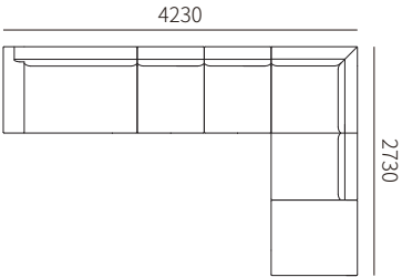
L186A-2R + L186B-2 + L186E-2R + L186E-D 4230*2730*720MM 166.5*107.5*28.3"
