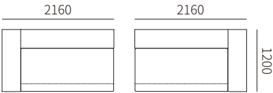
DA04A-2R 2160*1200*590MM 85.0*47.2*23.2"
