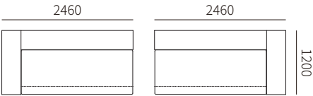
DA04A-3R 2460*1200*590MM 96.9*47.2*23.2"
