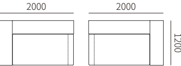
DA04C-1L 2000*1200*590MM 78.7*47.2*23.2"
