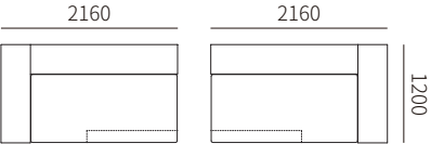
DA04E-2R 2160*1200*590MM 85.0*47.2*23.2"
