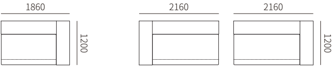
DA04A-1L 1860*1200*590MM 73.2*47.2*23.2"
