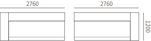
DA04A-4R 2760*1200*590MM 108.7*47.2*23.2"
