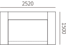
DA04-3A 2520*1500*590MM 99.2*59.1*23.2"
