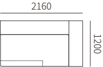
DA04E-2L 2160*1200*590MM 85.0*47.2*23.2"
